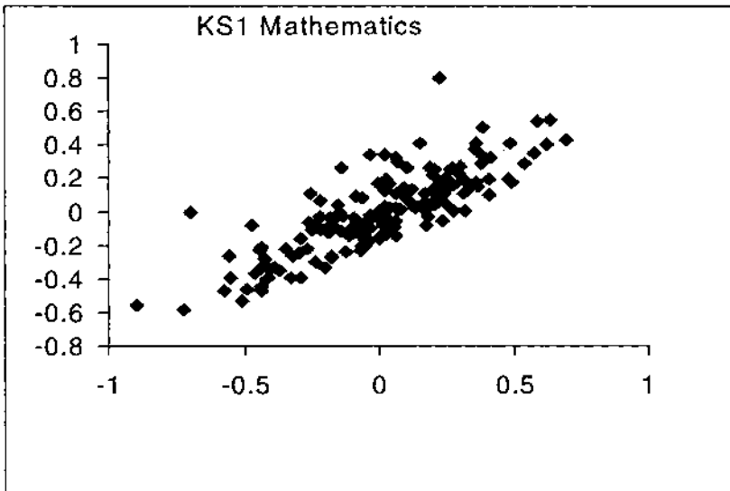
FIG. 2. School level residuals, for Mathematics, adjusted for all pupil and school level variables (Y axis) against residuals adjusted for baseline variables only (X axis). Correlation \approx 0.72 .
