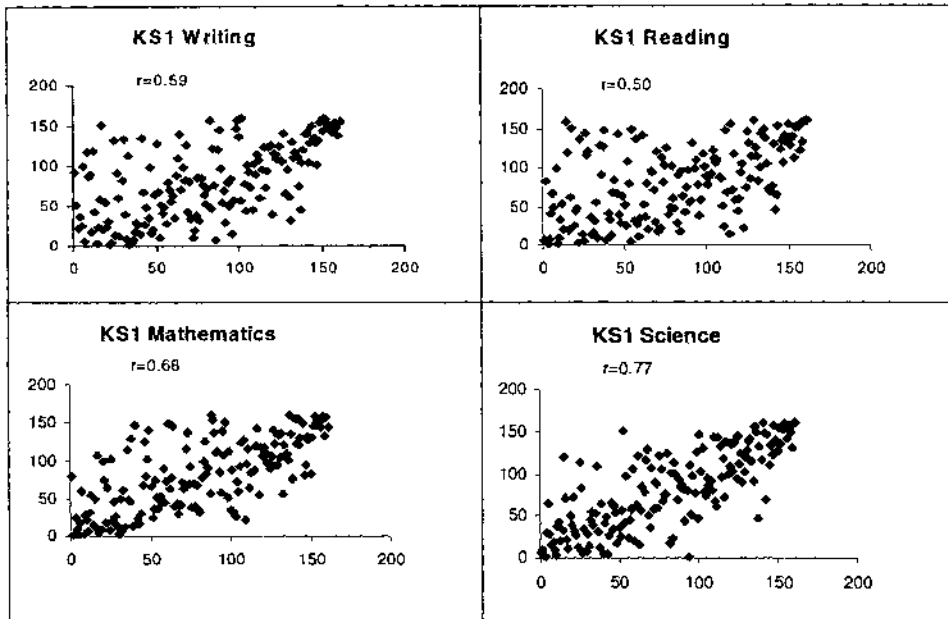
FIG. 1. Adjusted school level residuals (Y axis) by school raw means (X axis) for KS1 outcomes. The scale values are ranks.
