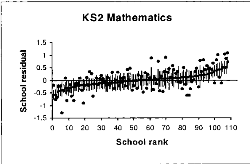
FIG. 4. KS2 Mathematics residual estimates, 95% confidence intervals and unadjusted mean scores.
