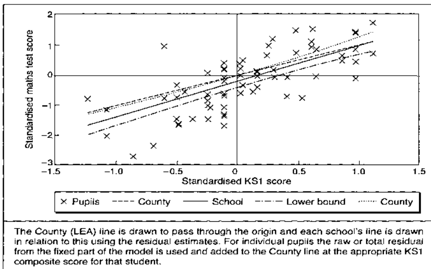
FIG. 5. A differential value added graph for one school for Mathematics outcome at KS2.
