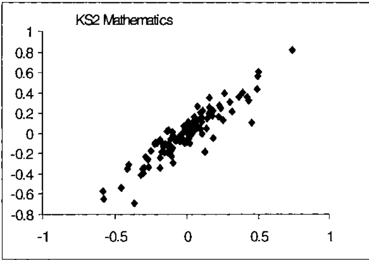
FIG. 3. School level residuals, for Mathematics, adjusted for all pupil level variables (Y axis) against residuals adjusted for KS1 variables only (X axis).
