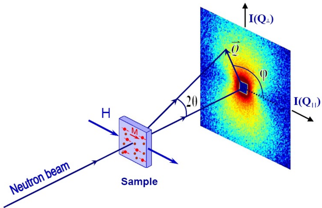
Figure 2: Small-angle neutron scattering characterising the nanoscale clusters in the Fe alloy. The anisotropic pattern arises from the spin dependent scattering of the magnetic contrast between the Cu cluster and the Fe alloy.
