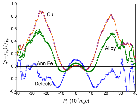
Figure 1: Positron annihilation spectrum as a function of the electron momentum p_L . The deformed Fe-Cu alloy response is composed of the reference curves for pure Cu, Fe and defects in Fe.
