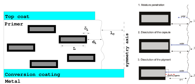
Figure 1: Left: schematic of a fractured organic coating that contains several encapsulated pigments dispersed through the primer. Right: response in a fractured coating -water uptake (top), capsule disruption (center), and leaching of corrosion inhibitors (bottom)- modelled in this study.
