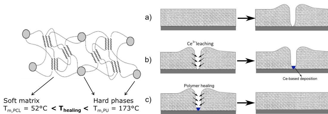
Figure 1: Physical structure of the cross-linked polymer network, and mechanism of multiple action self-healing: (a) Scratched coating, followed by (b) \text{Ce}^{3+} release and precipitation at defect site; (c) Thermally triggered healing of the scratch in the polymer material.
