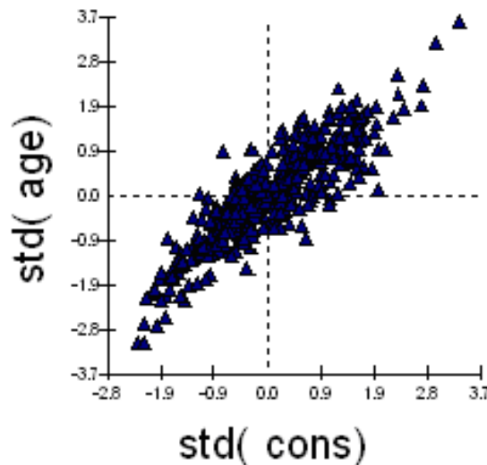
Level 2 standardised residual plot: slope vs. intercept
