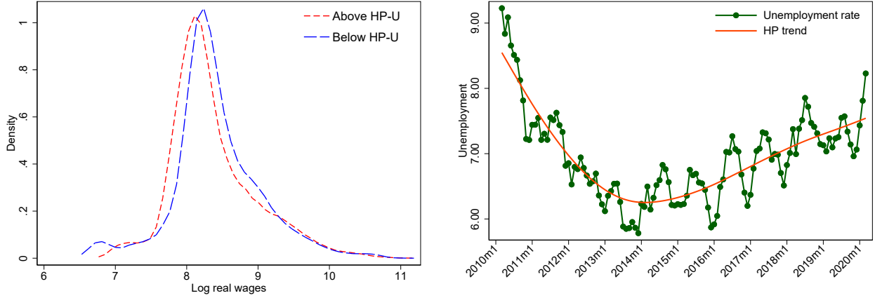
Figure 1: Histogram of log real wages (full time jobs), according to the aggregate unemployment rate trend deviation at the time of posting (left) and time series of unemployment rate. We also plot its Hodrick-Prescott smoothed trend with parameter \lambda = 14,400 as a reference (right).
