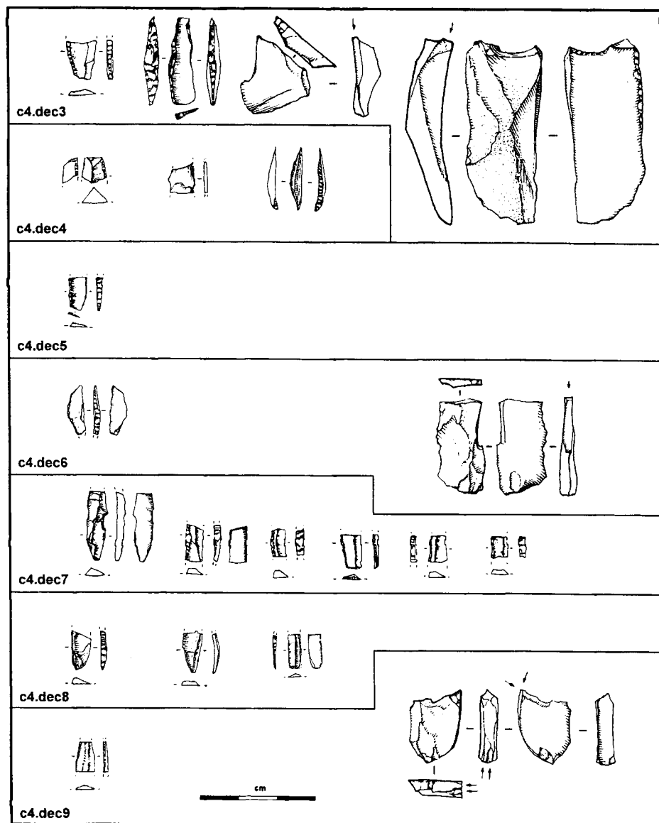
Figure 6. Salto do Boi (Cardina I), squares Q/15-16. Diagnostic tools (microliths and burins) in the 5 cm thick excavation units in which layer 4 was subdivided. In this section of the site, the following occupations were identified: dec 1-3, Terminal Magdalenian; dec 4-6, Late Gravettian with backed and truncated bladelets; dec 7-9, Gravettian with Noailles burins.
