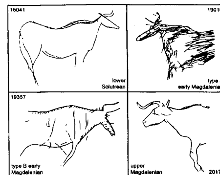
Stylistical evolution of the representations of aurochs and horse in the engraved stone slabs from Parpalló cave (Valencia)
