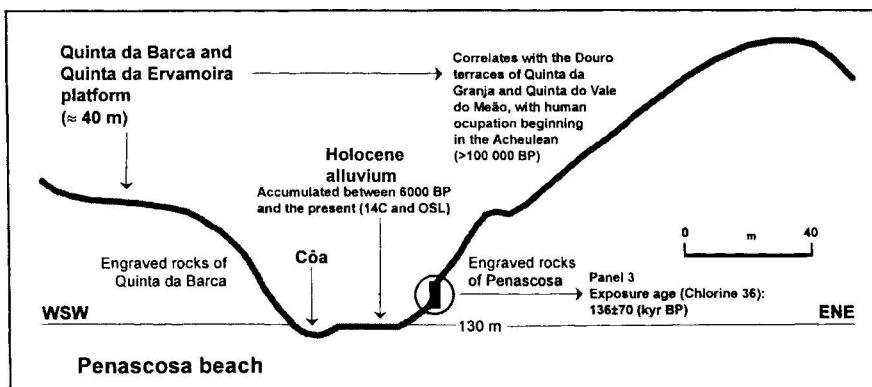
Figure 3. Terraces of the lower Côa and chronology of the valley's incision (see Fig. 7 for the location of the sites where the schematic profiles were obtained).
