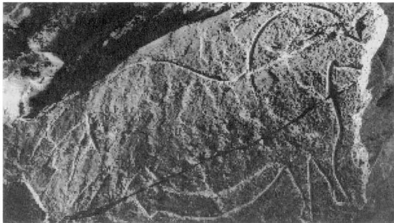
Figure 2. The Mazouco horse, the first open air Palaeolithic figure to be recognised as such by archaeologists (Jorge et al. 1981).
