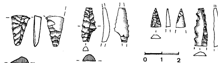
Figure 8. Olga Grande Sul. Diagnostic Upper Solutrean tool types: 1. stem of shouldered point; 2. shouldered point; 3. tip of shouldered point; 4. denticulated backed bladelet.
