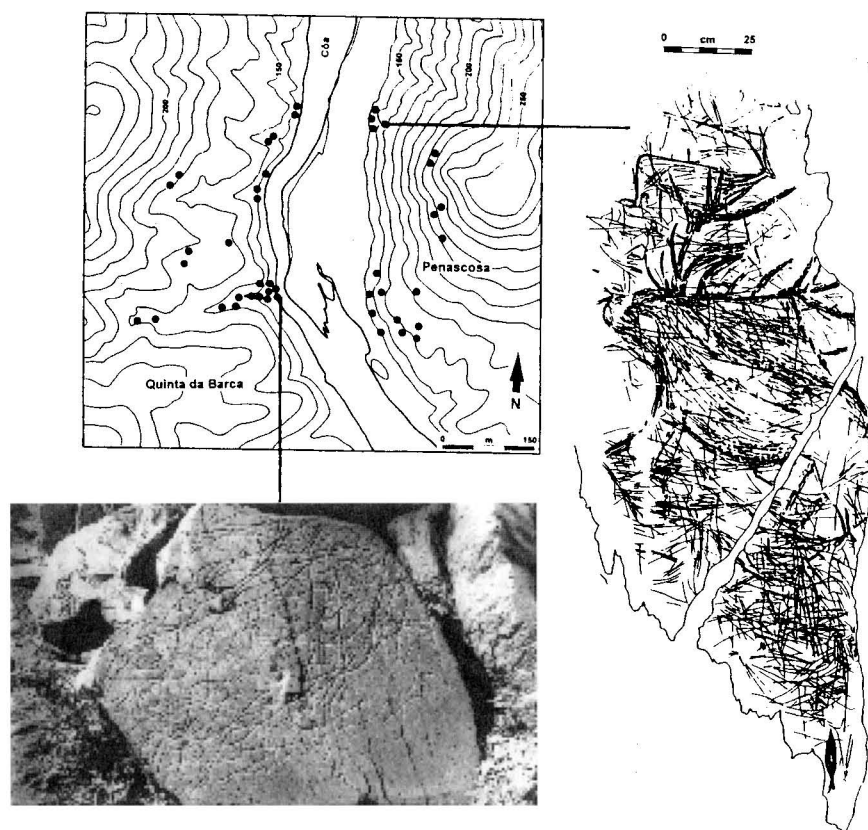
Figure 19. Distribution of known engraved rocks in Penascosa and Quinta da Barca. Palaeolithic art clusters in two main groups marking, on both sides of the river, the limits of a large sand beach, which coincide with outcrops of harder rocks. At the northern end, Panel 10 features a large number of incised and scraped figures, among which the large deer is illustrated on the right. At the southern end, the 'spaghetti rock', illustrated below the map, features an almost indecipherable superposition of a large number of pecked and abraded figures, among which a few horses and aurochs are more easily recognisable.
