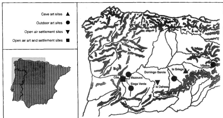
Figure 1. Upper Palaeolithic sites of the Douro basin. Cova valley and Mazouco are located in Portugal, the others in Spain.
